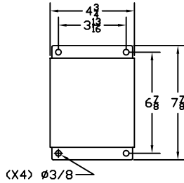
BRACKET FOOTPRINT
